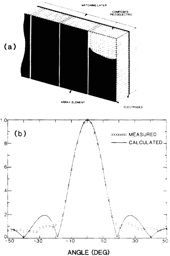
Figure 14. (a) Schematic representation of a composite linear array with elements defined by the electrode pattern alone and (b) the CW radiation pattern from a single element of such an array compared with the radiation pattern calculated for an isolated element of the same width (After Shaulov et al. [24]).
