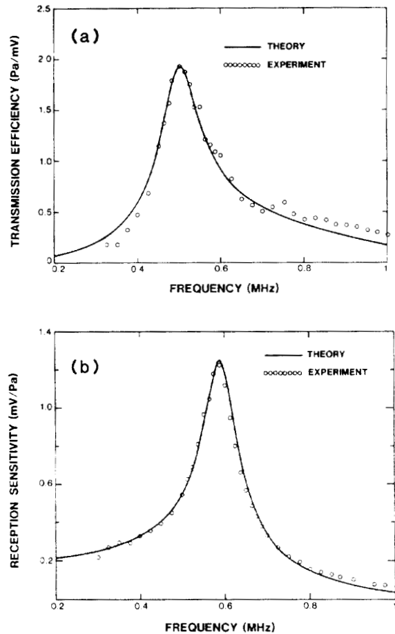
Figure 9. Absolute transmission efficiency and absolute reception sensitivity measured on a composite disk along with theoretical fits. The material parameters used in these fits agree well with those determined from the resonance in the electrical impedance (After Smith et al. [17]).
